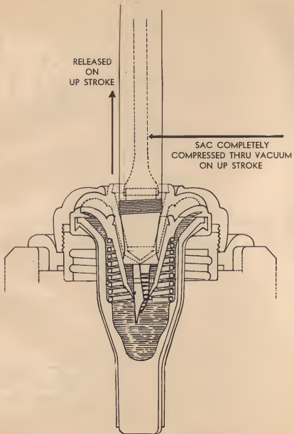
THIRD—Pen released, Penfiller evacuating air completely.
